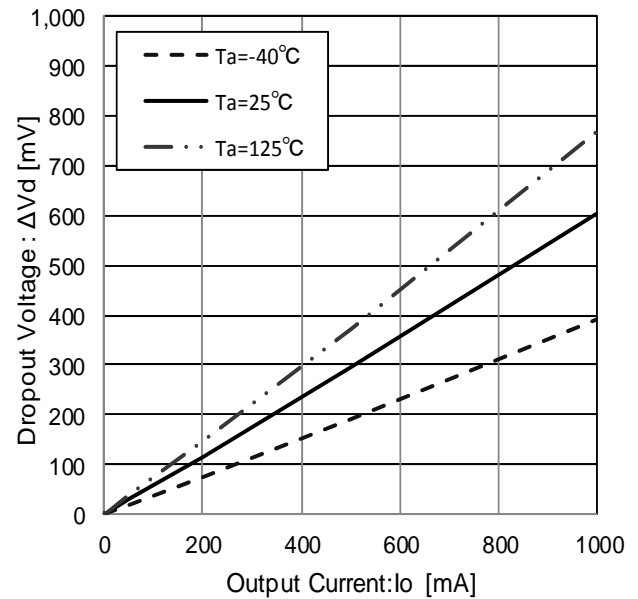
Figure 39. Dropout Voltage ( V_{cc} = V_o \times 0.95\text{V} )
