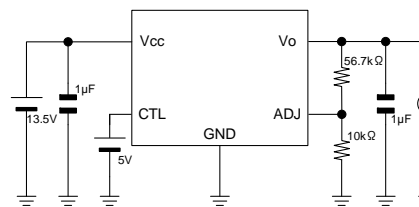
Measurement setup for Figure 22
