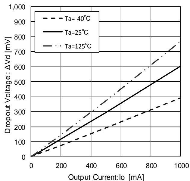
Figure 16. Dropout Voltage ( V_{CC}=V_{Ox0.95} , 0mA \leq I_O \leq 1000mA )
