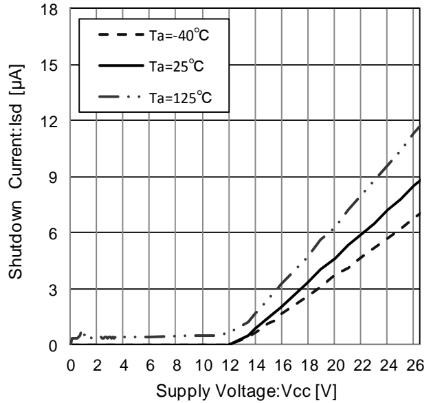
Figure 12. Shutdown Current
