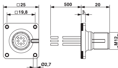
Dimensional drawing
