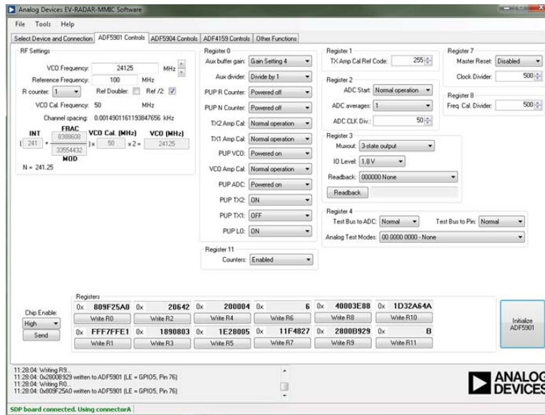
Figure 4. ADF5901 Controls
