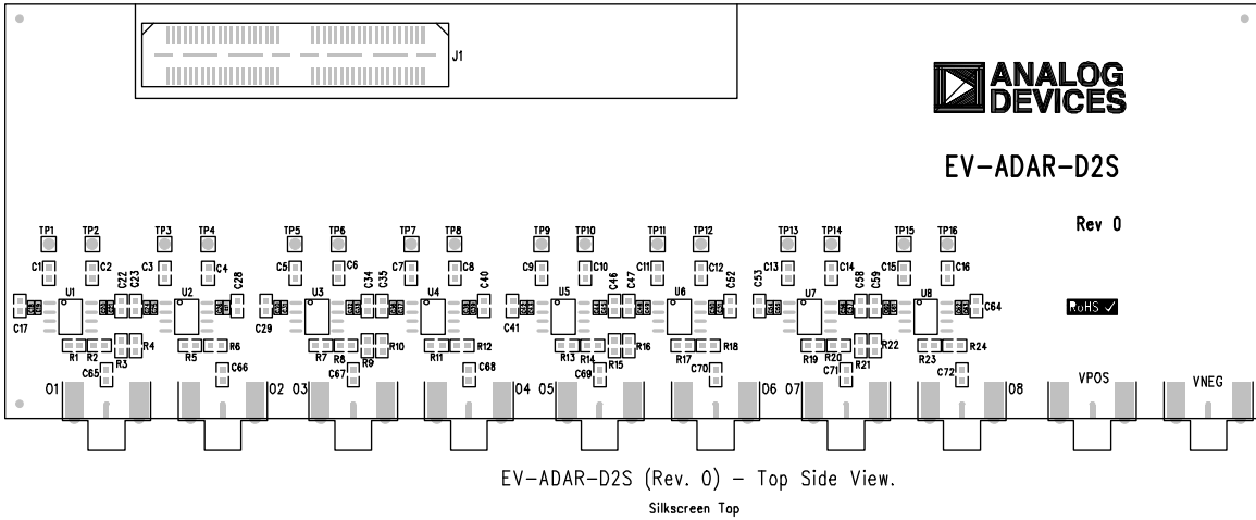
Figure 31. EV-ADAR-D2S Assembly
