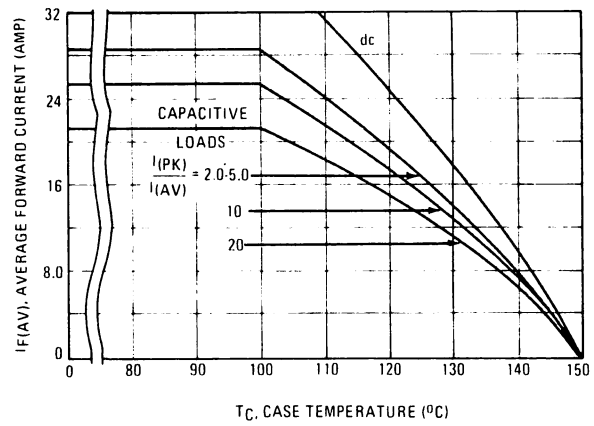
FIGURE 7 – CURRENT DERATING
