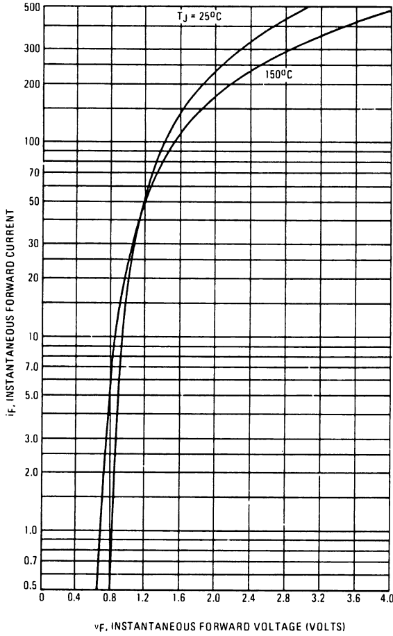
FIGURE 1 – FORWARD VOLTAGE
