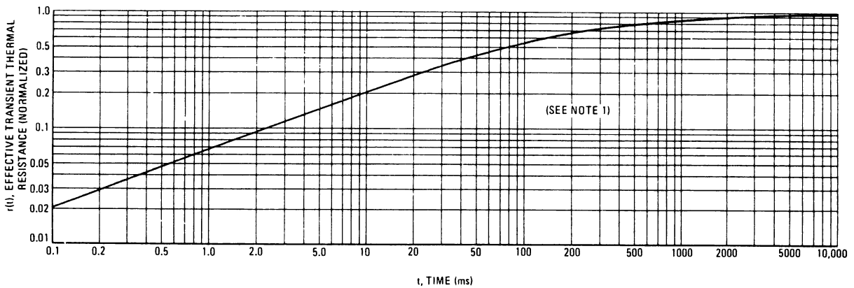
FIGURE 3 – THERMAL RESPONSE
