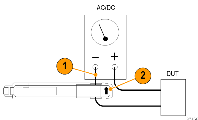
Figure 8: Current probe polarity
