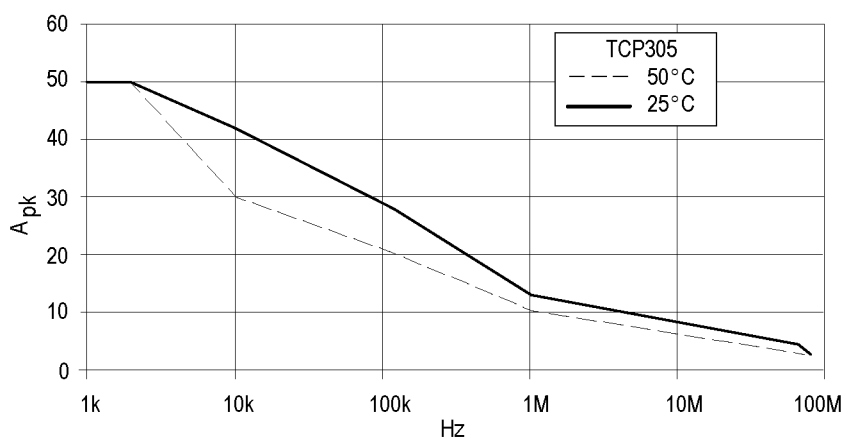
Figure 29: Frequency derating-TCP305
