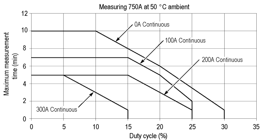
Figure 34: Measuring 750A noncontinuous at 50 °C ambient temperature
