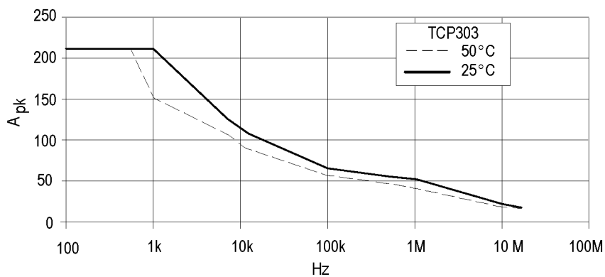
Figure 30: Frequency derating-TCP303
