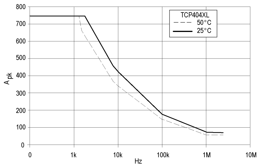
Figure 31: Frequency derating-TCP404XL
