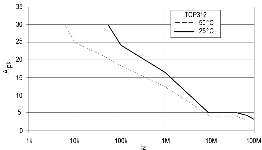
Figure 28: Frequency derating-TCP312
