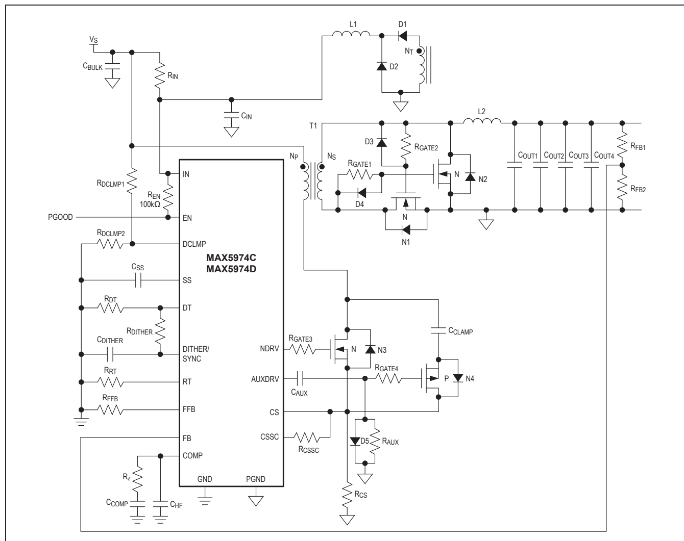
Typical Application Circuits (continued)
