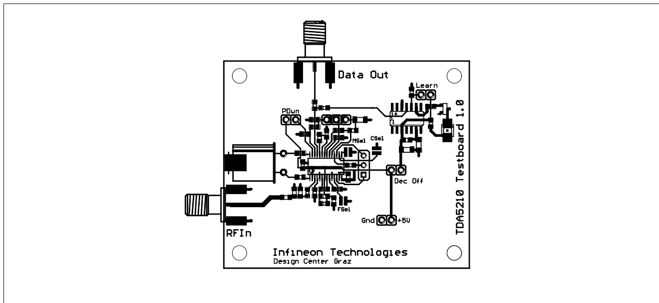
Figure 12 Top Side of the Evaluation Board
