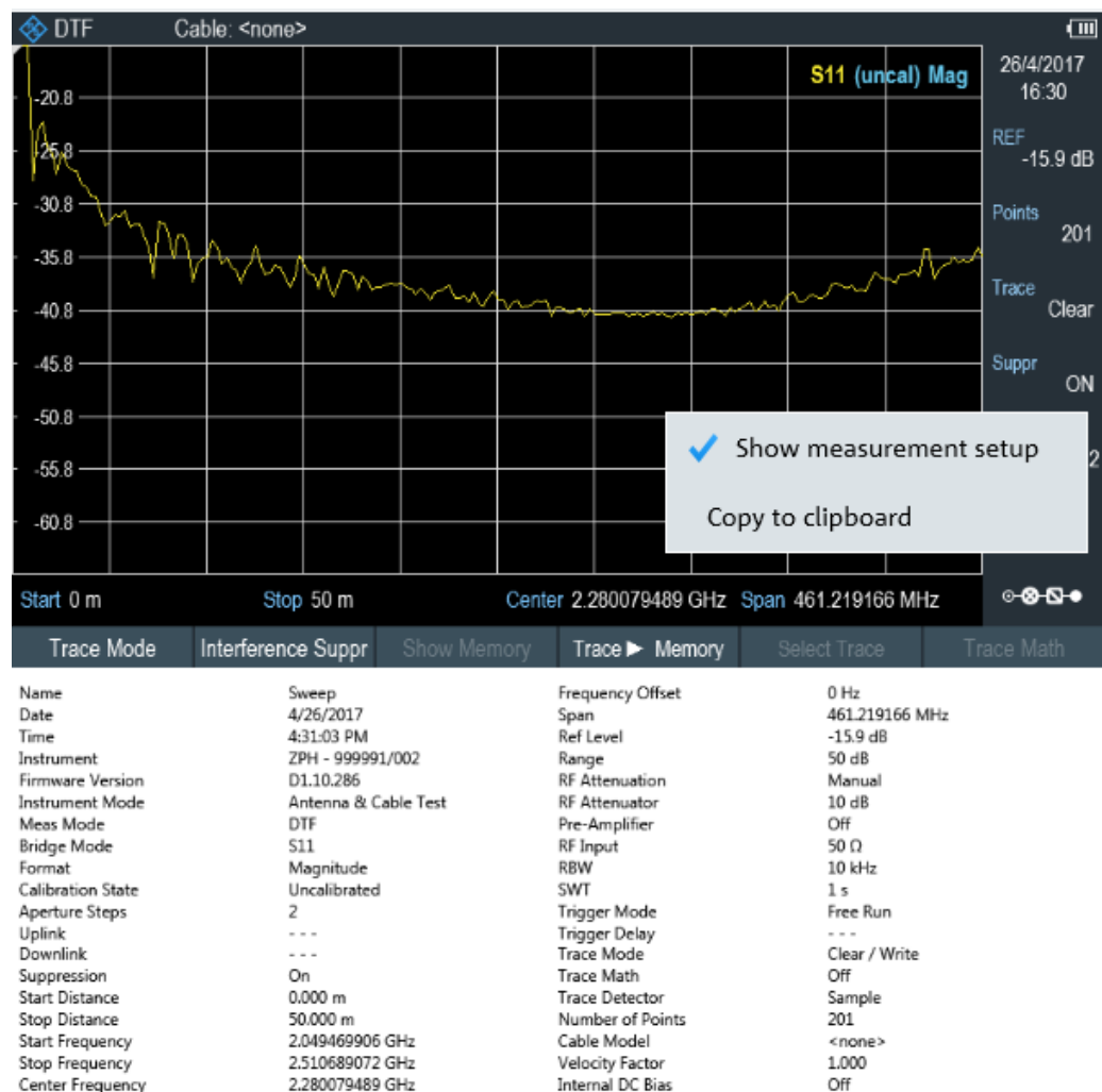
Figure 4-15: Screenshot
