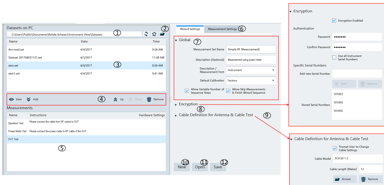
Figure 4-32: Wizard editor
