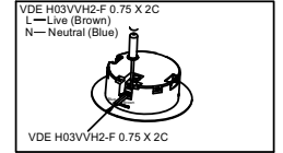
③ Feed the power cable through the mounting hole and connect to terminal block on fixture.
