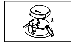
④ Fixed cable locker. Connect battery connector, Snap battery pack on housing.
