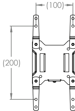
MOUNTING PROFILE
