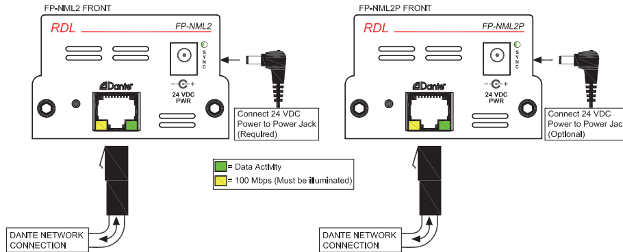
Audio and Power Bus Connections
