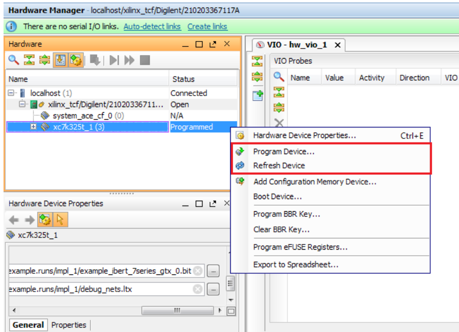
Figure 1-14: Program/Refresh Device
