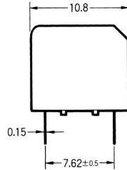
Side Actuator (long-lever)
