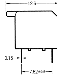
Side Actuator (short-lever)
