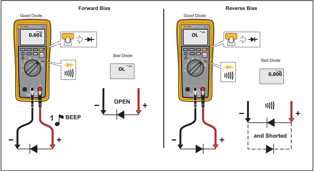
Figure 7. Diode Test
