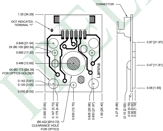
ATLAS attached to EZ-Connect EZ-4000-0357
