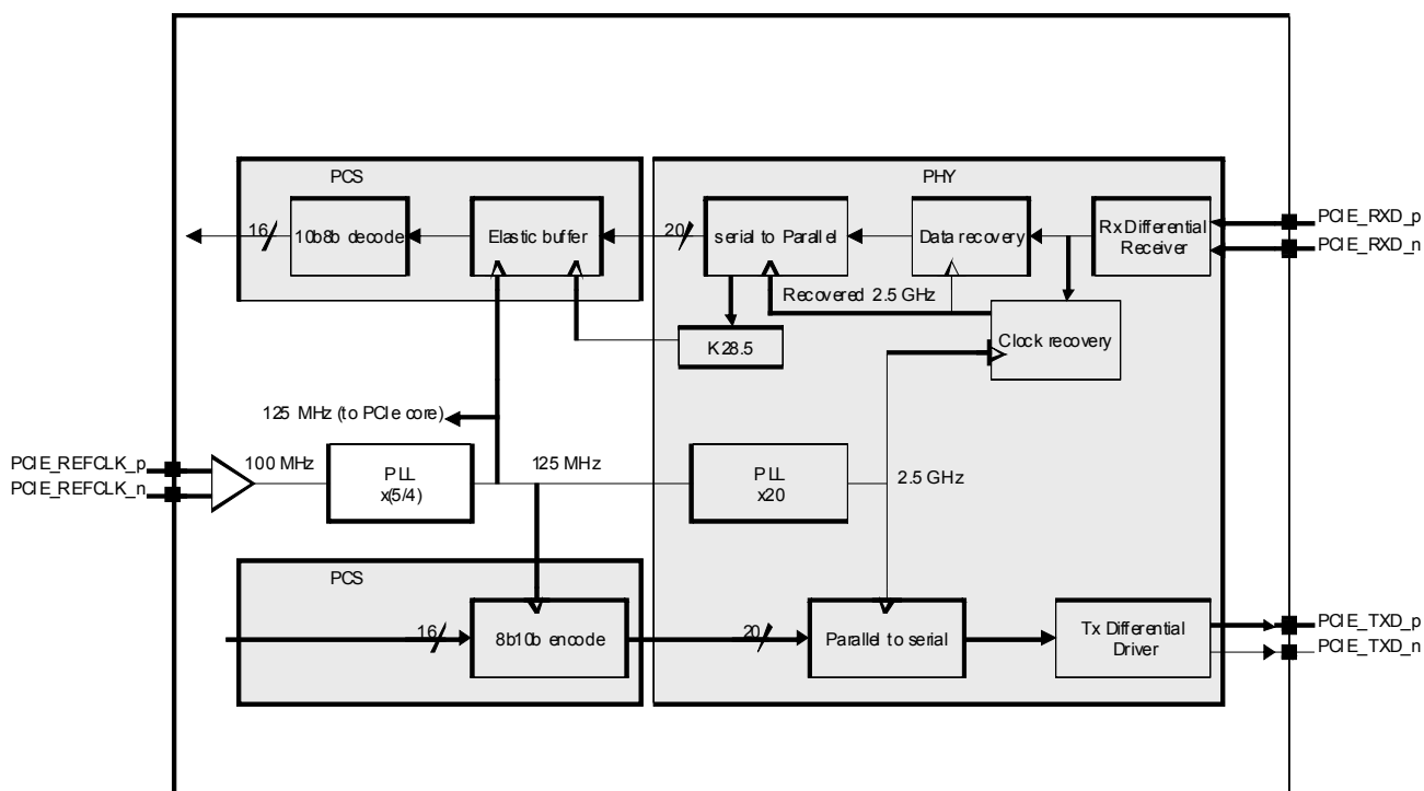
Figure 24: PCIe Clocking
