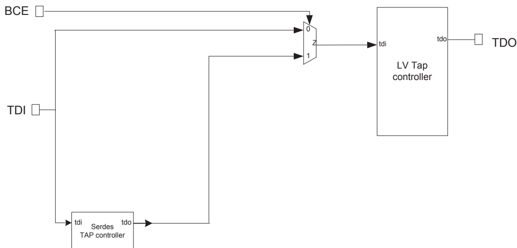
Figure 37: PCIe SerDes Connections
