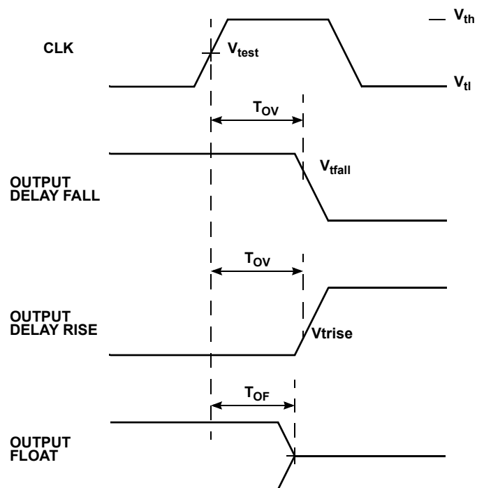
Figure 42: Output Timing Measurement Waveforms
