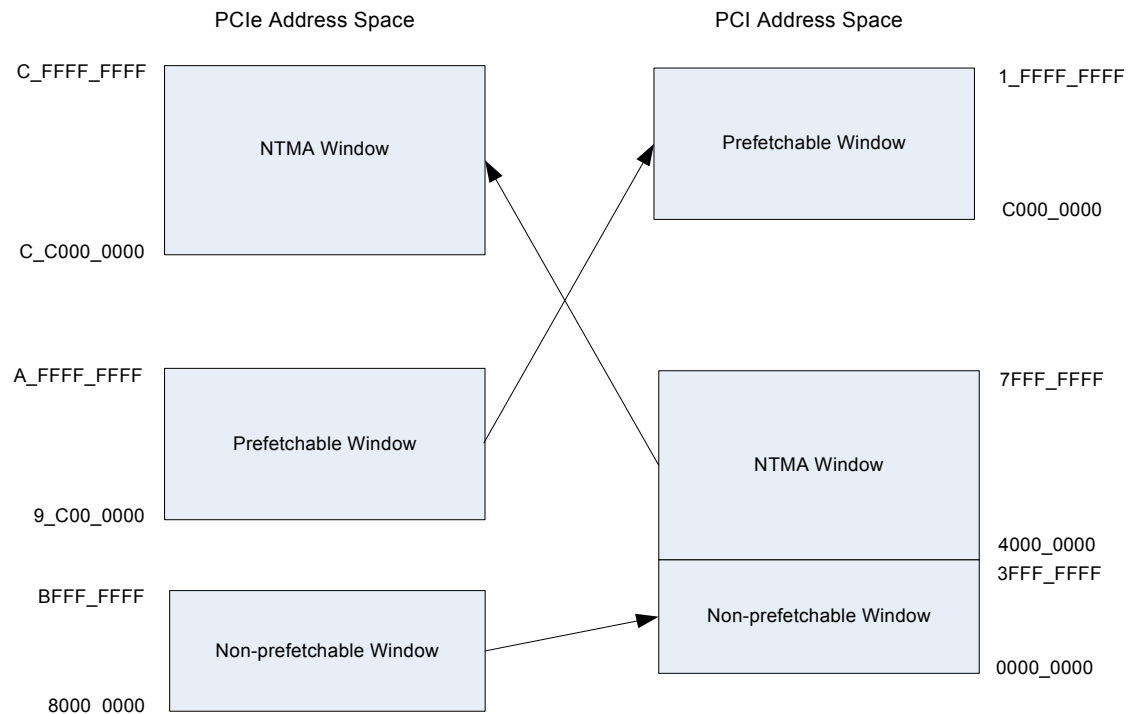
Figure 11: Memory Window Remapping Example
