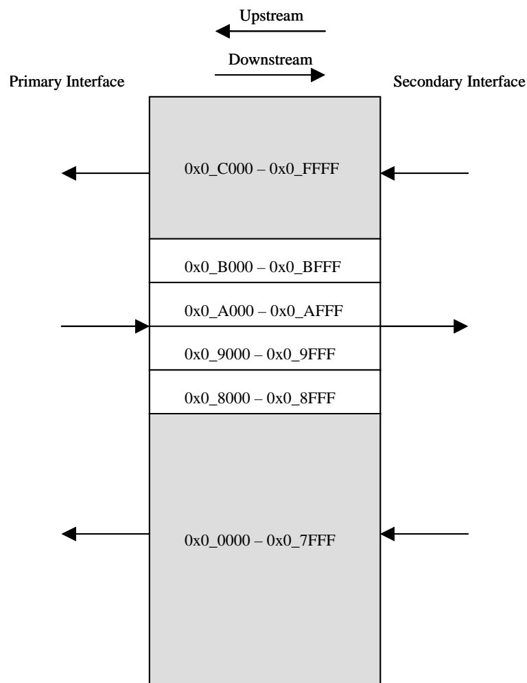
Figure 9: I/O Address Space
