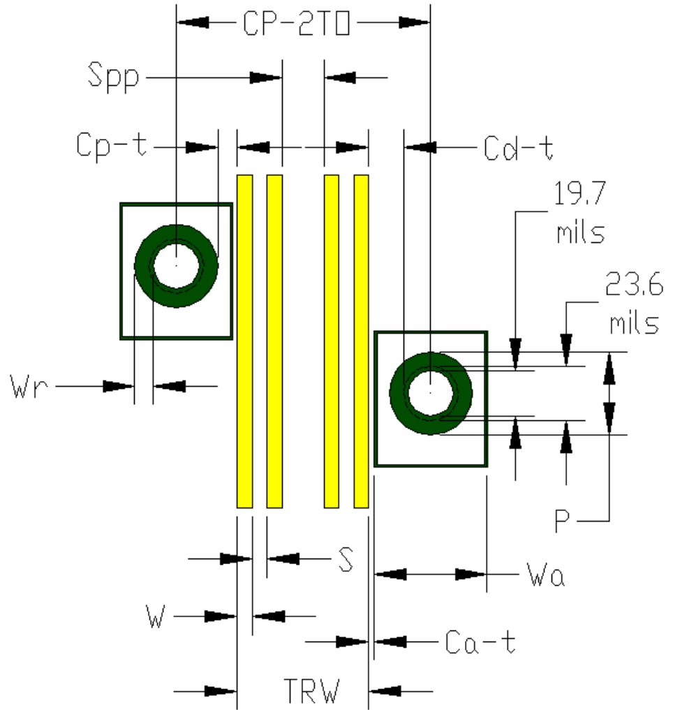
Figure 12: Orthogonal Header PCB trace routing example, 4.2mm pitch between columns
