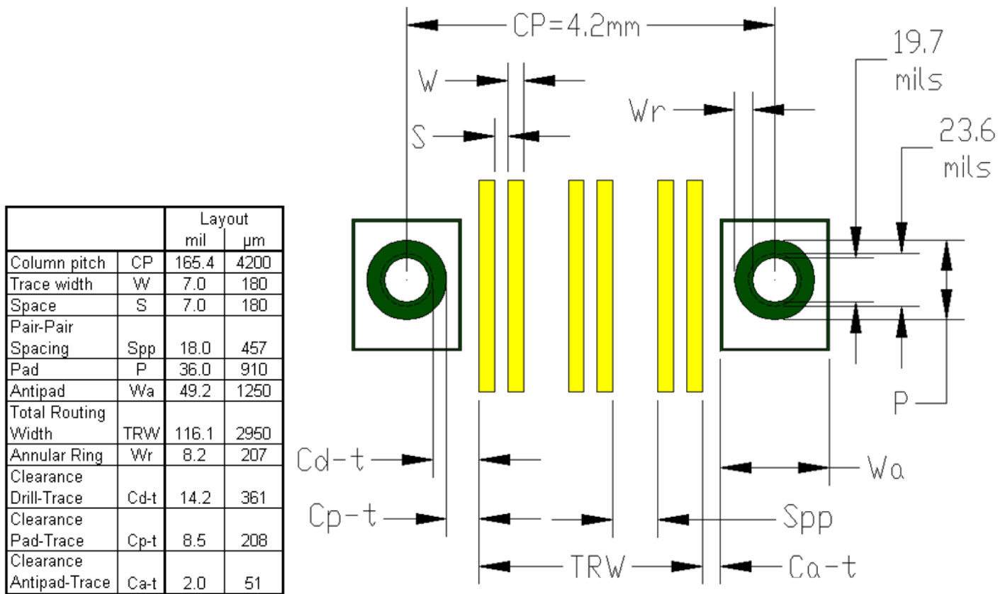
Figure 11: Orthogonal RAR PCB trace routing example, 4.2mm pitch between columns
