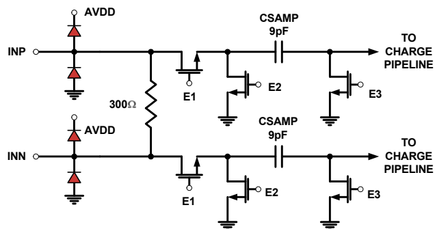
FIGURE 42. ANALOG INPUTS
