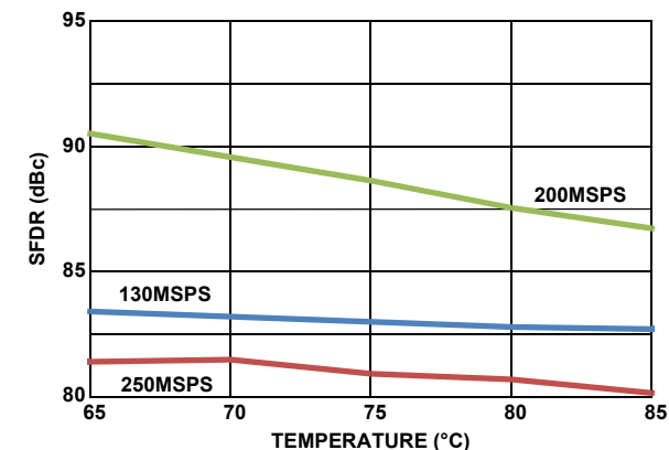
FIGURE 25. TYPICAL SFDR PERFORMANCE vs TEMPERATURE, DEVICE CALIBRATED AT +85^{\circ}\text{C} , f_{\text{IN}} = 105\text{MHz} , -2\text{dBFS}
