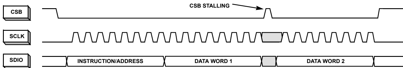
FIGURE 39. 2-BYTE TRANSFER
