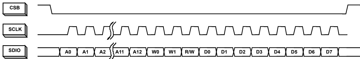
FIGURE 36. LSB-FIRST ADDRESSING
