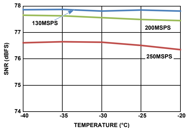
FIGURE 20. TYPICAL SNR PERFORMANCE vs TEMPERATURE, DEVICE CALIBRATED AT -40^{\circ}\text{C} , f_{\text{IN}} = 105\text{MHz} , -2\text{dBFS}
