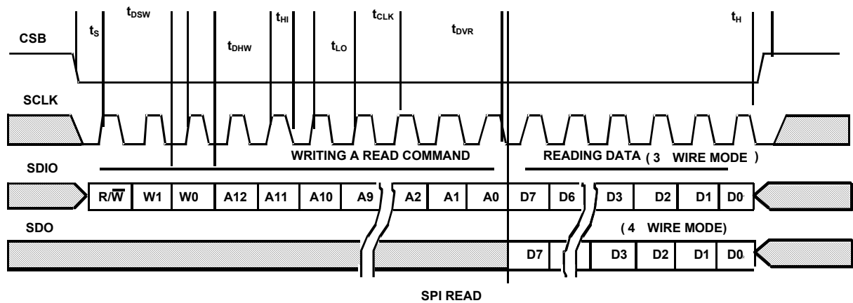
FIGURE 38. SPI READ
