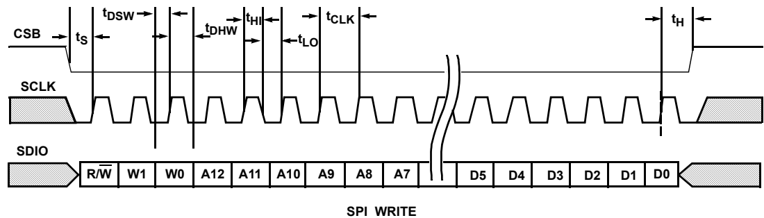
FIGURE 37. SPI WRITE
