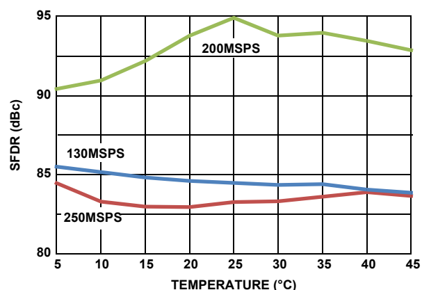
FIGURE 23. TYPICAL SFDR PERFORMANCE vs TEMPERATURE, DEVICE CALIBRATED AT +25^{\circ}\text{C} , f_{\text{IN}} = 105\text{MHz} , -2\text{dBFS}
