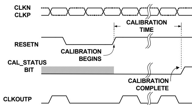
FIGURE 19. CALIBRATION TIMING
