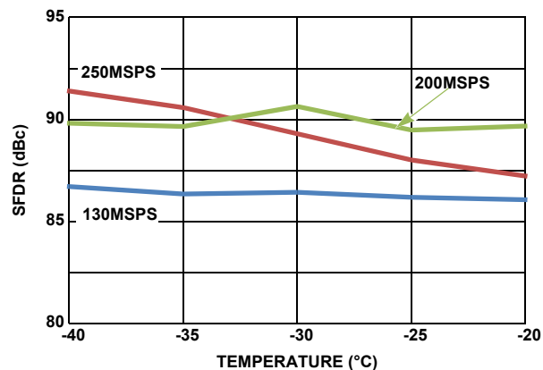
FIGURE 21. TYPICAL SFDR PERFORMANCE vs TEMPERATURE, DEVICE CALIBRATED AT -40^{\circ}\text{C} , f_{\text{IN}} = 105\text{MHz} , -2\text{dBFS}
