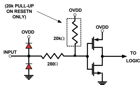
FIGURE 45. DIGITAL INPUTS
