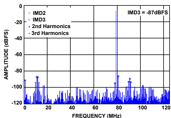
FIGURE 17. TWO-TONE SPECTRUM (F1 = 170MHz, F2 = 171MHz AT -7dBFS)
