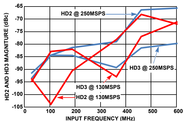
FIGURE 3. HD2 AND HD3 vs f_{IN}
