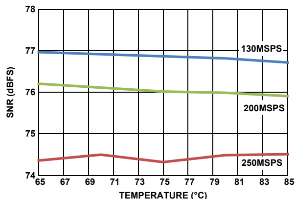
FIGURE 24. TYPICAL SNR PERFORMANCE vs TEMPERATURE, DEVICE CALIBRATED AT +85^{\circ}\text{C} , f_{\text{IN}} = 105\text{MHz} , -2\text{dBFS}
