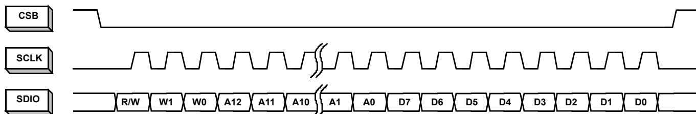
FIGURE 35. MSB-FIRST ADDRESSING
