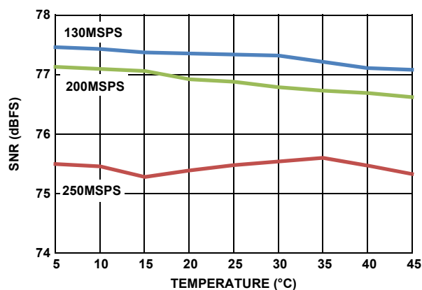
FIGURE 22. TYPICAL SNR PERFORMANCE vs TEMPERATURE, DEVICE CALIBRATED AT +25^{\circ}\text{C} , f_{\text{IN}} = 105\text{MHz} , -2\text{dBFS}
