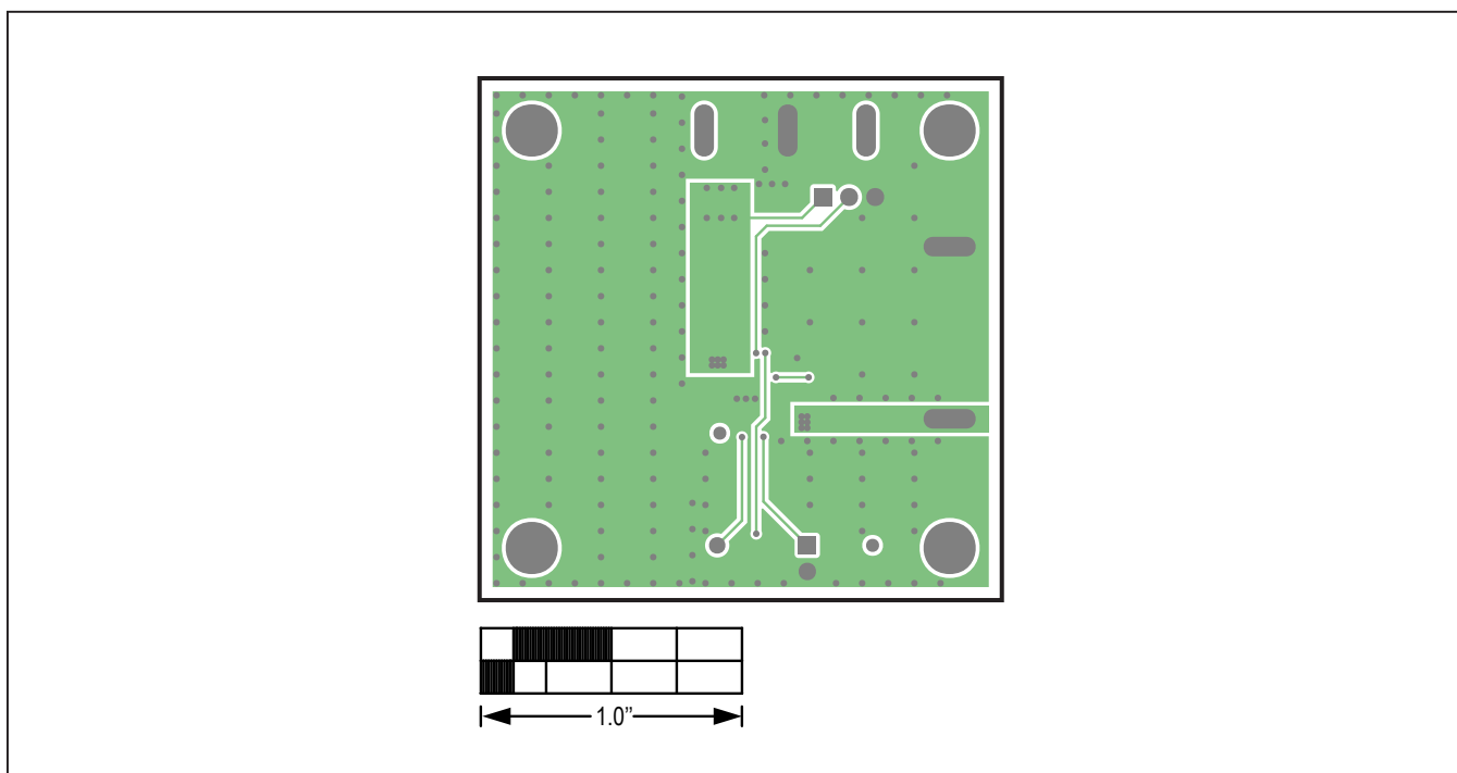
MAXM15462 EV Kit PCB Layout—Layer 3 Power
