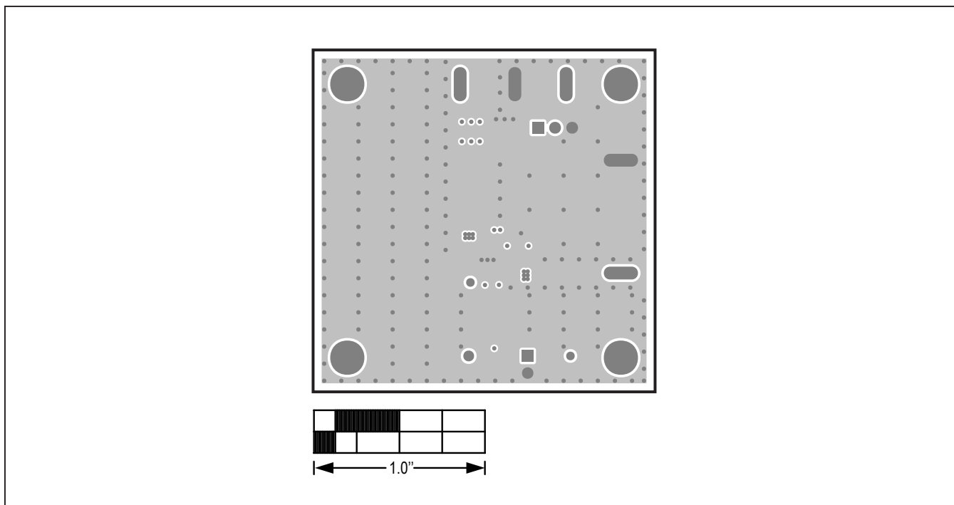
MAXM15462 EV Kit PCB Layout—Layer 2 Ground
