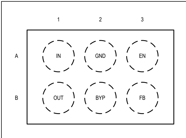
MAX38902C
