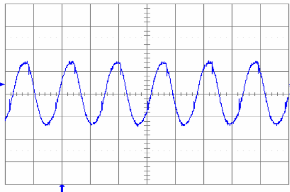
Fig. 1.8V.6: Output voltage ripple (20 mV/div.) at full rated load current into a resistive load with external capacitance 10 \mu\text{F} ceramic + 1 \mu\text{F} ceramic and V_{in} = 5 \text{ V} for V_{out} = 1.8 \text{ V} . Time scale: 2 \mu\text{s} /div.
