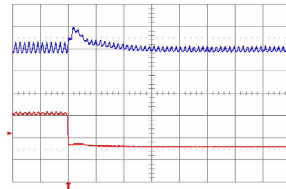
Fig. 1.0V.8: Output voltage response for V_{out} = 1.0 V to negative load current step change from 5 A to 2.5 A with slew rate of -5 A/ \mu s at V_{in} = 5 V. Top trace: output voltage (100 mV/div.); Bottom trace: load current (2 A/div.). C_o = 47 \mu F ceramic + 1 \mu F ceramic. Time scale: 20 \mu s/div.
