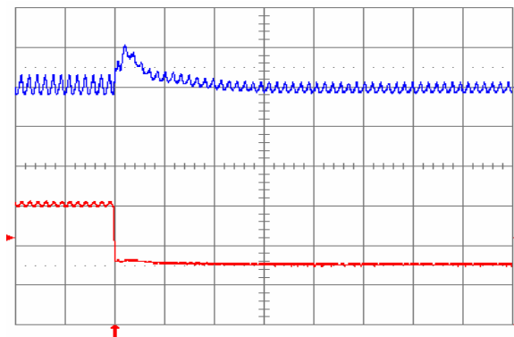
Fig. 1.2V.8: Output voltage response for V_{out} = 1.2 V to negative load current step change from 5 A to 2.5 A with slew rate of -5 A/ \mu s at V_{in} = 5 V. Top trace: output voltage (100 mV/div.); Bottom trace: load current (2 A/div.). C_o = 47 \mu F ceramic + 1 \mu F ceramic. Time scale: 20 \mu s/div.
