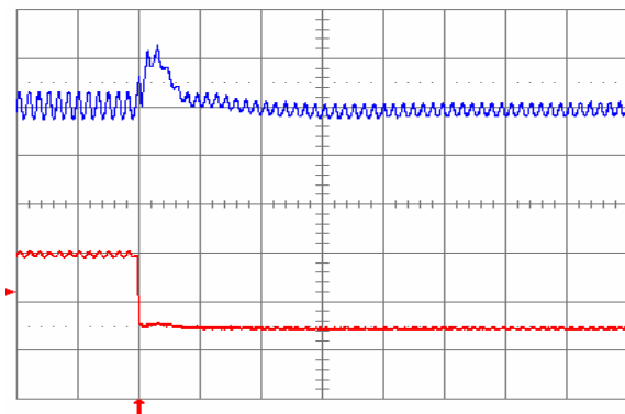
Fig. 1.8V.8: Output voltage response for V_{out} = 1.8 \text{ V} to negative load current step change from 5 A to 2.5 A with slew rate of -5 \text{ A}/\mu\text{s} at V_{in} = 5 \text{ V} . Top trace: output voltage (100 mV/div.); Bottom trace: load current (2 A/div.). C_o = 47 \mu\text{F} ceramic + 1 \mu\text{F} ceramic. Time scale: 20 \mu\text{s} /div.
