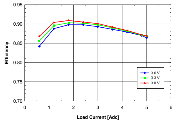
Fig. 1.2V.4: Efficiency vs. load current and input voltage for V_{out} = 1.2 V converter mounted vertically with air flowing from pin 5 to pin 1 at a rate of 200 LFM (1m/s) and T_a = 25 °C.
