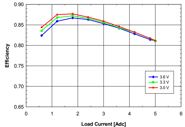
Fig. 0.7525V.4: Efficiency vs. load current and input voltage for V_{out} = 0.7525 V converter mounted vertically with air flowing from pin 5 to pin 1 at a rate of 200 LFM (1 m/s) and T_a = 25 °C.
