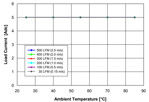
Fig. 0.7525V.2: Available load current vs. ambient temperature and airflow rates for V_{out} = 0.7525 V converter mounted horizontally with V_{in} = 5 V, air flowing from pin 5 to pin 1 and maximum MOSFET temperature \leq 120 °C.
