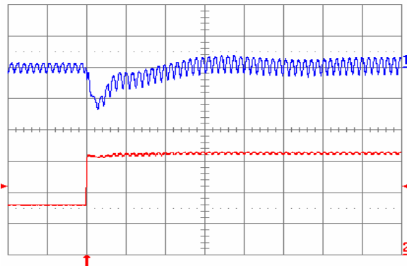
Fig. 3.3V.7: Output voltage response for V_{out} = 3.3 V to positive load current step change from 2.5 A to 5 A with slew rate of 5 A/ \mu s at V_{in} = 5 V. Top trace: output voltage (100 mV/div.); Bottom trace: load current (2 A/div.). C_o = 47 \mu F ceramic + 1 \mu F ceramic. Time scale: 20 \mu s/div.
