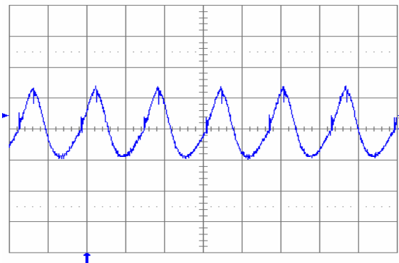
Fig. 1.0V.6: Output voltage ripple (20 mV/div.) at full rated load current into a resistive load with external capacitance 10 \mu F ceramic + 1 \mu F ceramic and V_{in} = 5 V for V_{out} = 1.0 V. Time scale: 2 \mu s/div.
