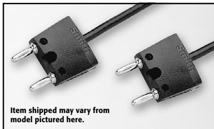
Model 8542-301: 1.2m (4 ft) shielded cable terminated with a dual banana plug on each end. For use with binding post inputs or dual banana jacks.
