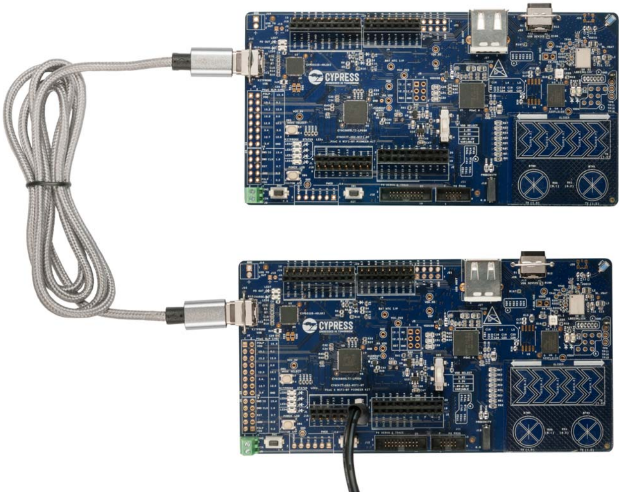
Figure A-3. EZ-PD CCG3 Power Delivery Setup using Two CY8CKIT-062-WiFi-BT Kits
