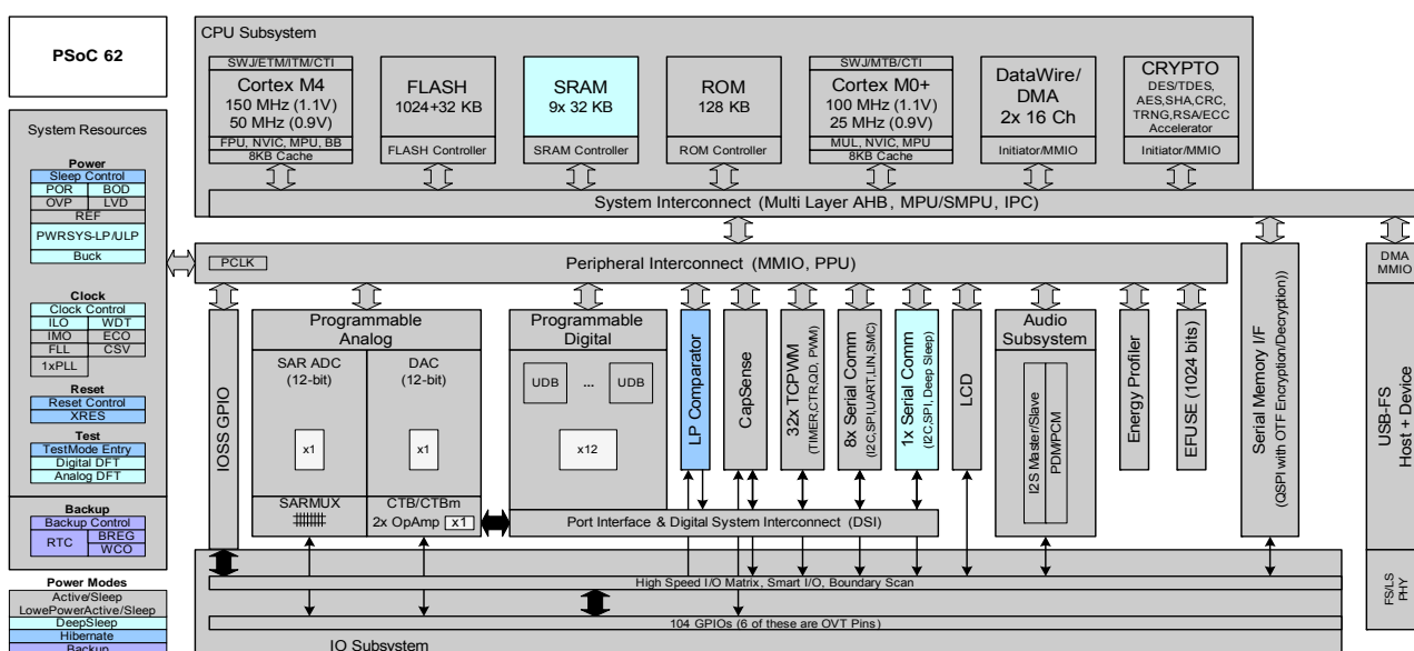
Figure 4-1. PSoC 6 MCU Block Diagram
