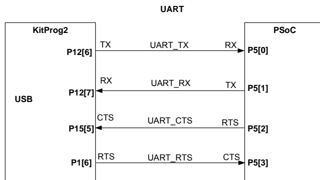
Figure 4-8. UART Connection between KitProg2 and PSoC 6
