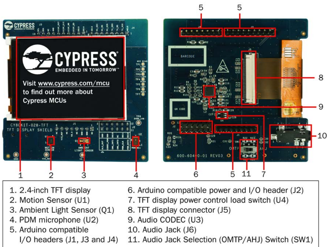
Figure 1-3. TFT Display Shield
