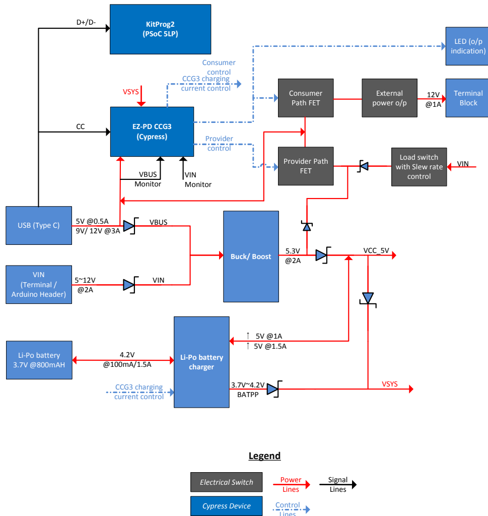
Figure 4-11. Type-C Block Diagram
