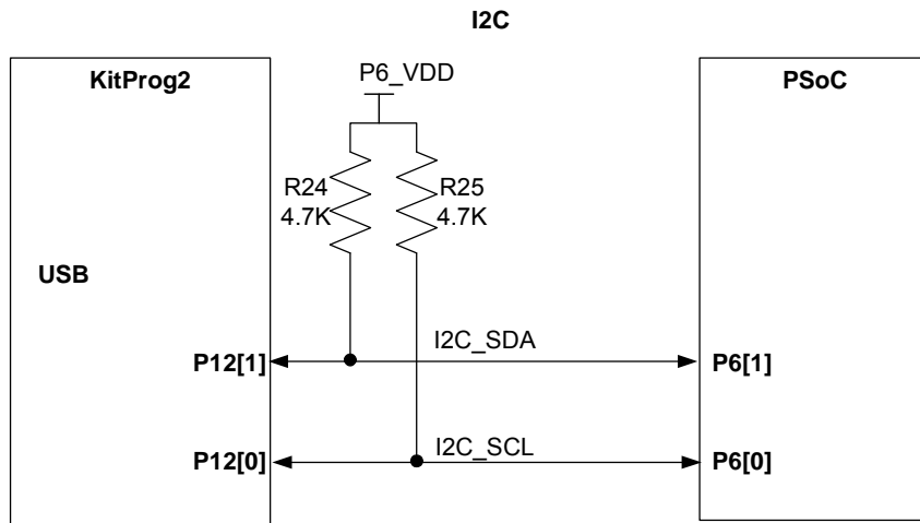
Figure 4-9. I2C Connection between KitProg2 and PSoC 6
