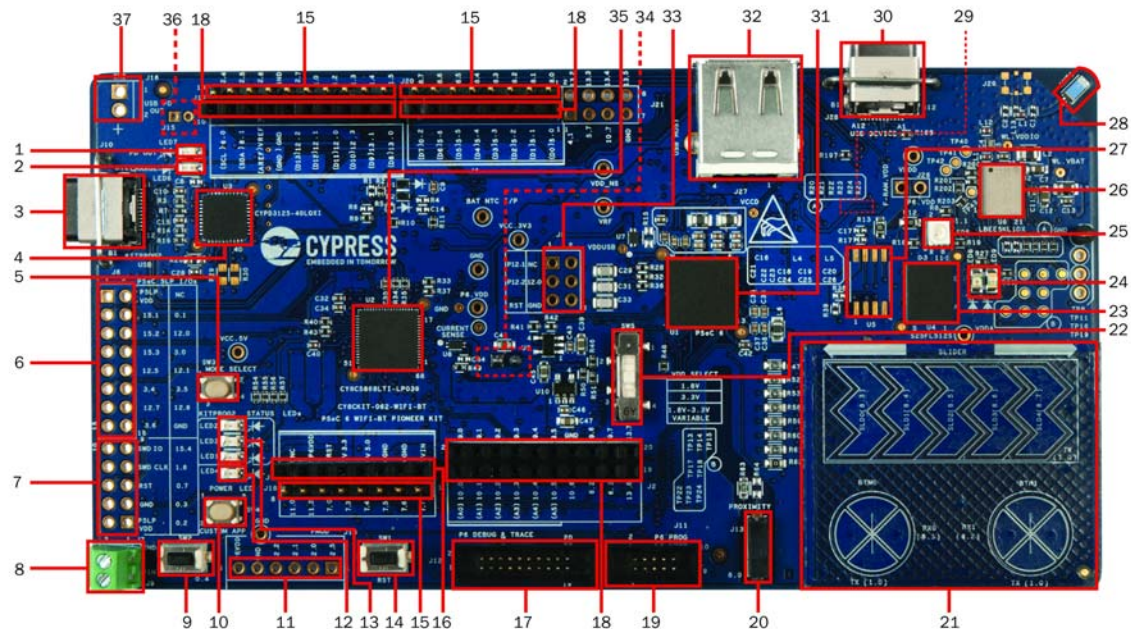
Figure 1-2. Pioneer Board
