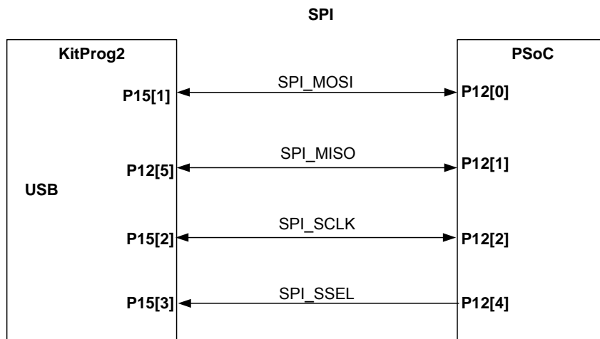
Figure 4-10. SPI Connection between KitProg2 and PSoC 6
