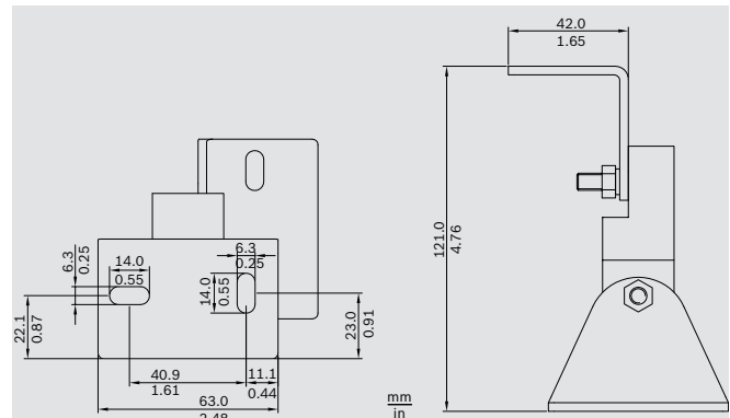
Bracket dimensions
