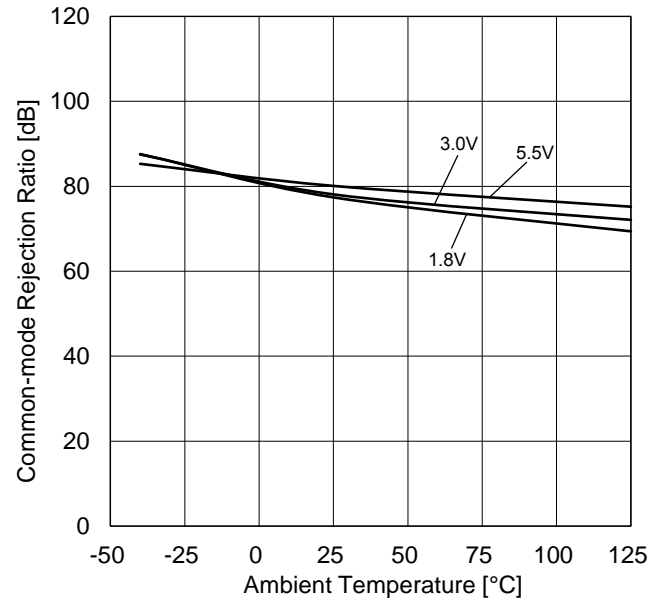
Figure 21. Common-mode Rejection Ratio vs Ambient Temperature
