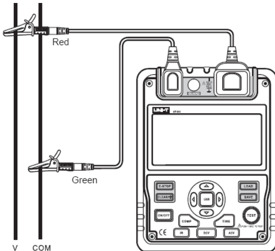
Figure 4. Voltage Measurement
