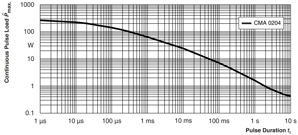
Maximum pulse load, continuous pulse; applicable if \bar{P} \leq P(\theta_{amb}) and \hat{U} \leq 2 kV; for permissible resistance change \pm (0.5 \% R + 0.05 \Omega)
