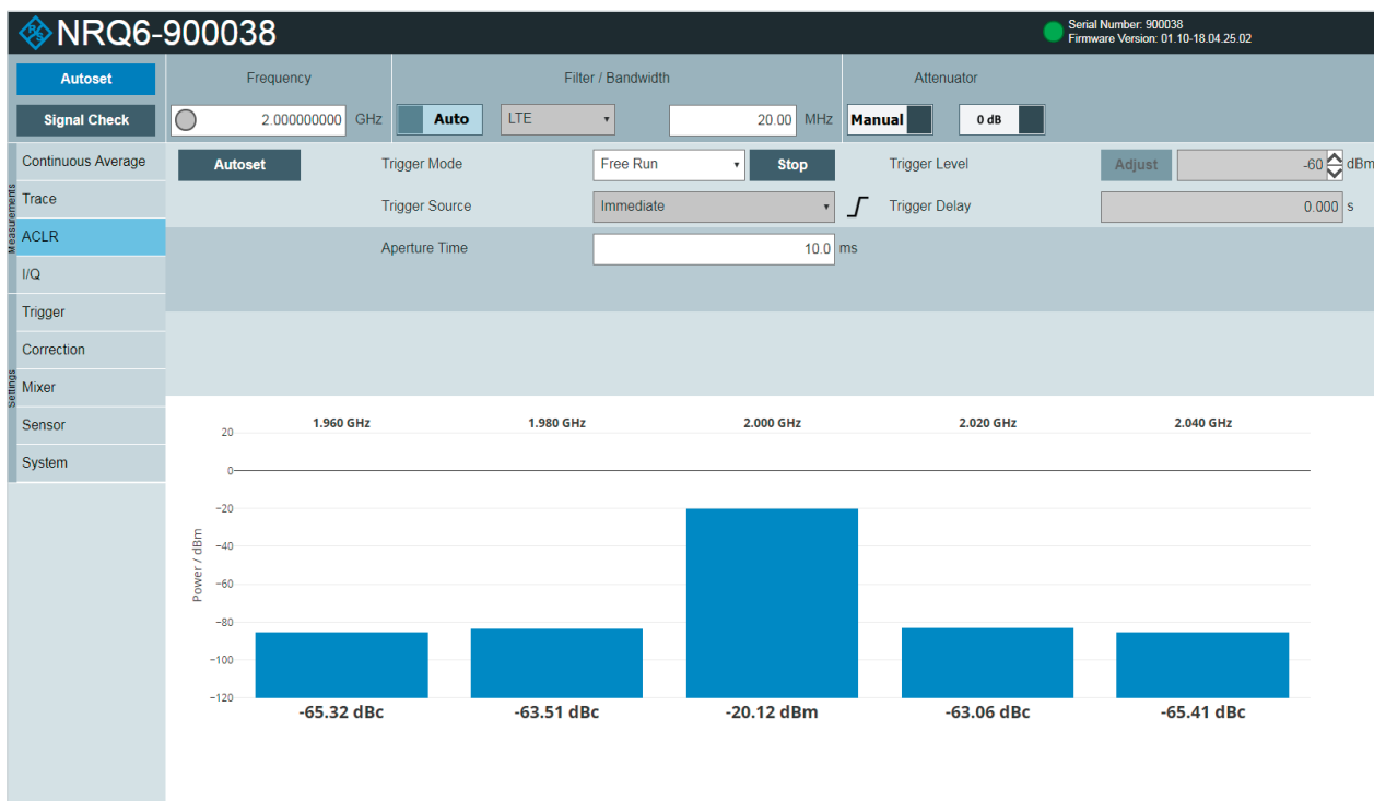
ACLR measurement on a 3.84 MHz 3GPP signal.
