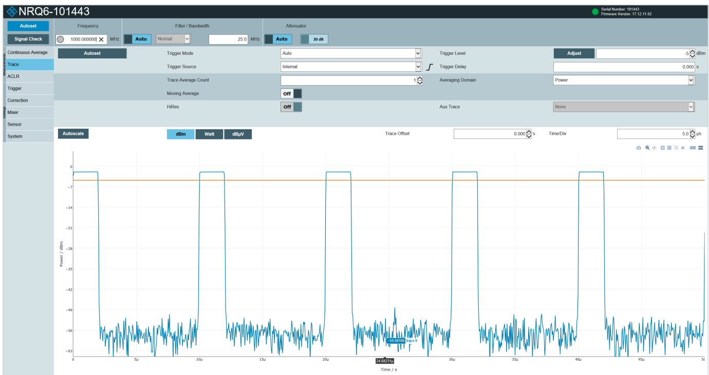
Trace measurement on a pulsed signal.
