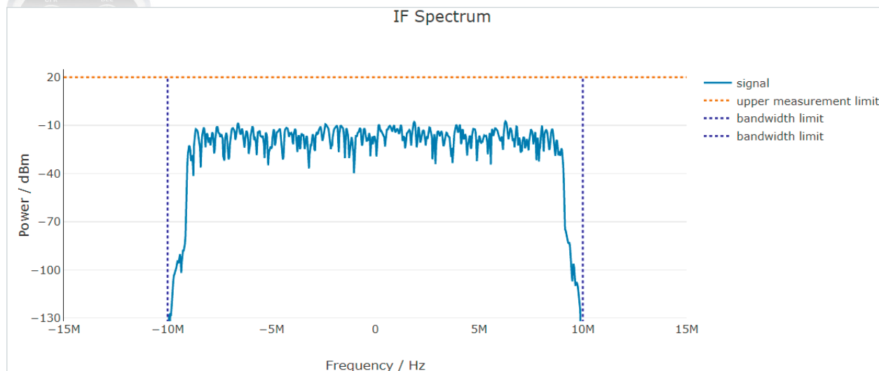
Signal check for a 20 MHz LTE signal.
