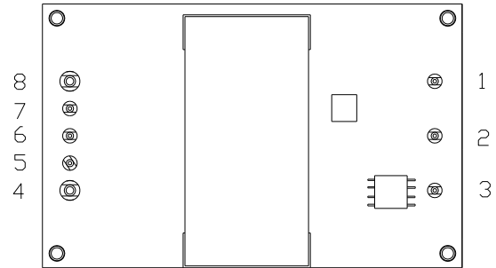
PIN CONNECTIONS
