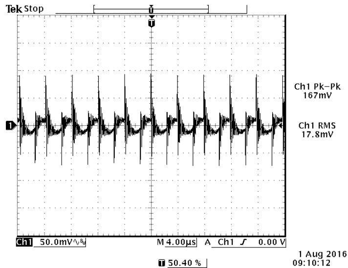
Ripple and noise 110Vdc input, 12Vdc/16.7A output and Ta=25 deg C, and with a 1uF ceramic cap and 220uF electrolytic cap at output.
