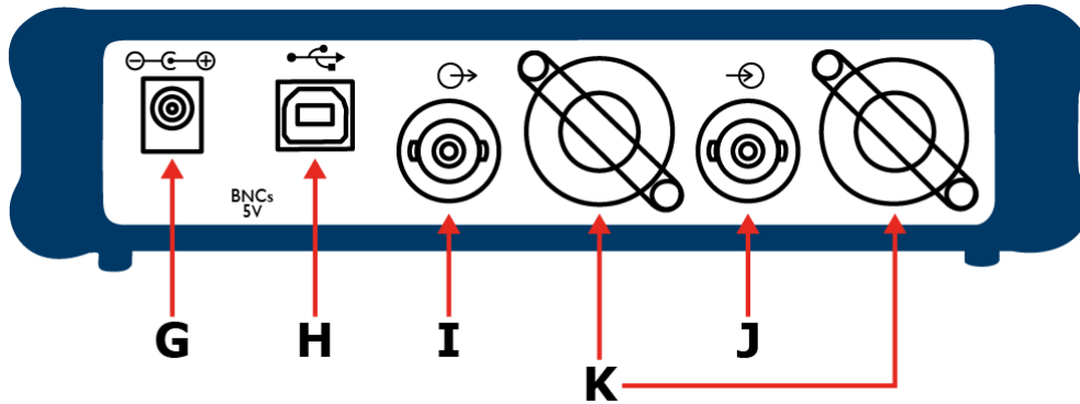
Rear panel: A and B models
