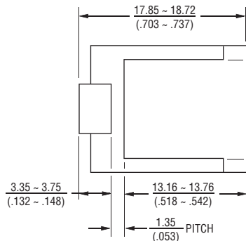
Existing Terminal Layout
