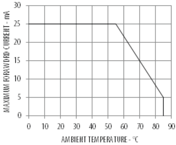
Figure 7 Derating Curve
