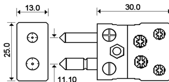
FAR019/0313. Standard Quick Wire Plugs
