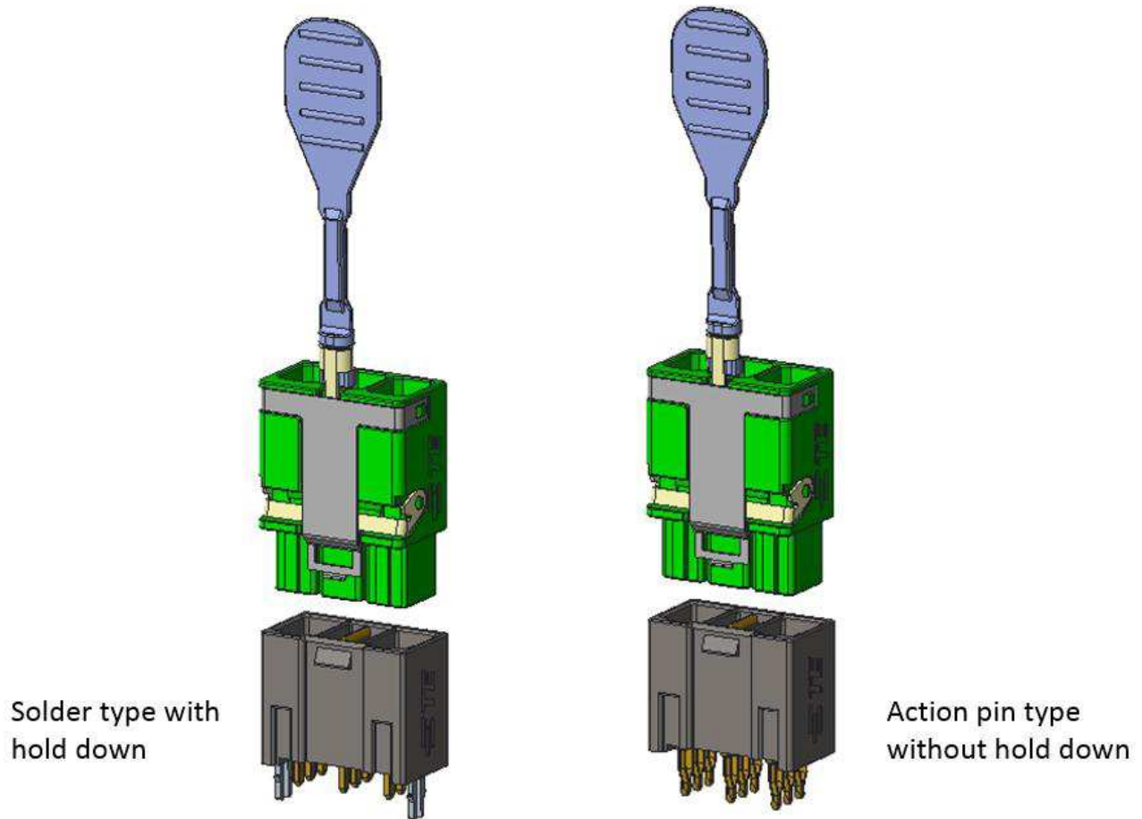
Figure 3, illustration of vertical board connector 2204585-x and cable connector 2204534-x (x means that different part number will be assigned for different plating or contact type)
