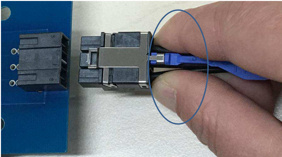
Figure 3 Correct mating procedure
