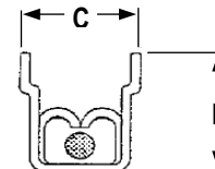
Section Y-Y: P/N 177916, 177914, 179592-1. and 179594-1
