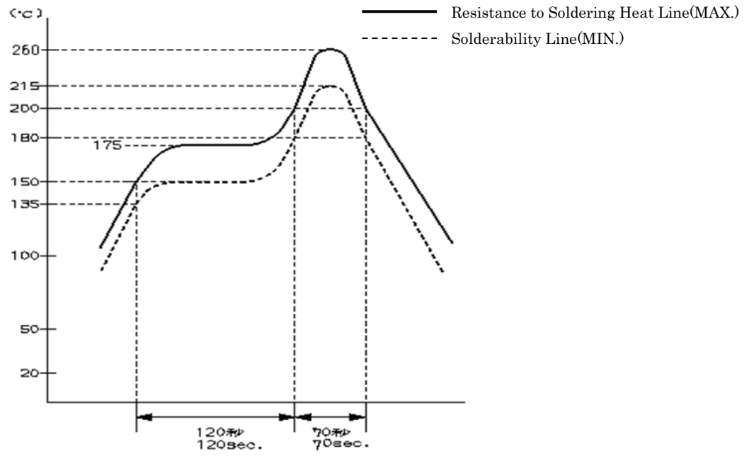
Fig. 3 Reflow Condition
