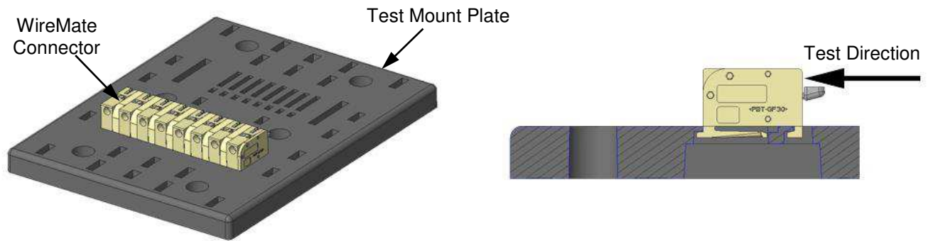
Figure 6 – Connector retention
