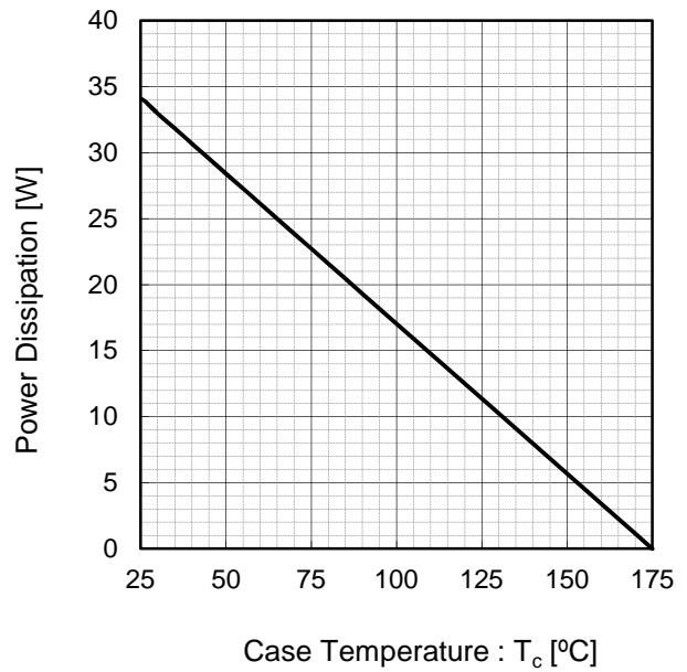
Fig.6 Power Dissipation
