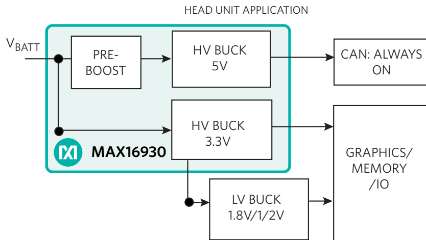
Figure 3. The MAX16930 provides an example of a dual buck with preboost and 20μA quiescent current. The preboost enables robust CAN bus operation during cold crank and start up. Low quiescent current minimizes the amount of discharge in the car battery during standby. The device operates 180 degrees out-of-phase at frequencies up to 2.2MHz to allow small external components, reduced output ripple, and to guarantee no AM band interference. To minimize EMI, the device provides a spread-spectrum option. The MAX16930 can be used for navigation and radio head units, as well as automotive power applications.
