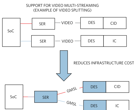
Figure 1. The ability to split video streams from an SoC allows a single data stream to be split into multiple streams to drive multiple displays in an automotive information cluster (IC) and the central information display (CID).
