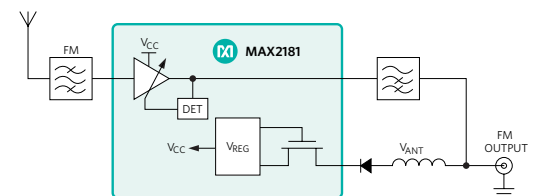
Figure 5. Simplified block diagram of MAX2181, an example of a highly integrated FM variable-gain low-noise amplifier for automotive FM and FM-diversity active antenna applications.
