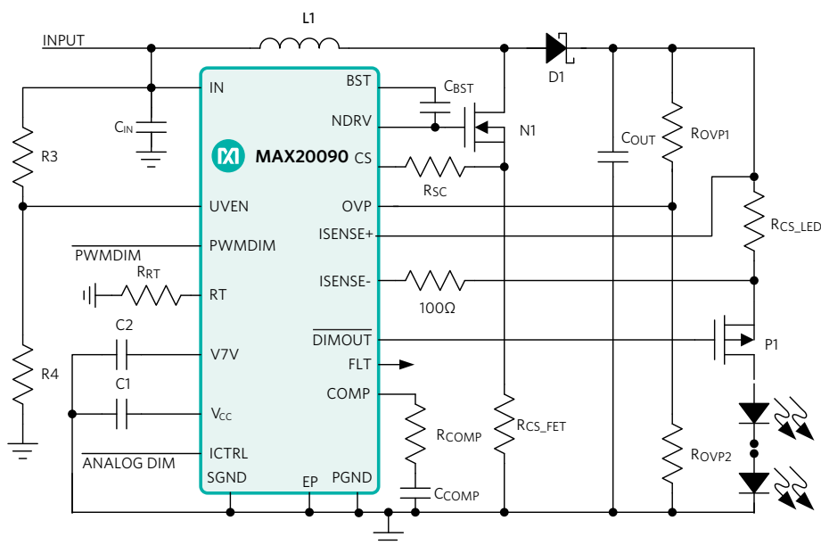
Figure 4. Typical operating circuit of the MAX20090, which is ideal for automotive front-light applications such as high beam, low beam, and daytime running lights.
