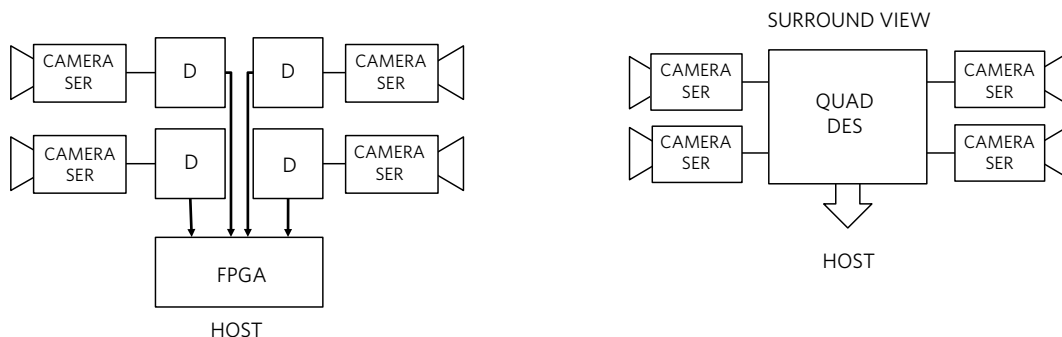
Figure 2. Video aggregation example.
