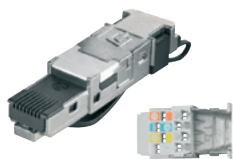
IP20-RJ45: field assembly connectors for Ethernet or PROFINET for use in control cabinets
