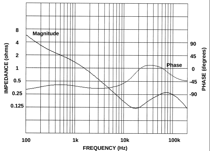
Model N6762A, CC Mode, @50V, 2A
