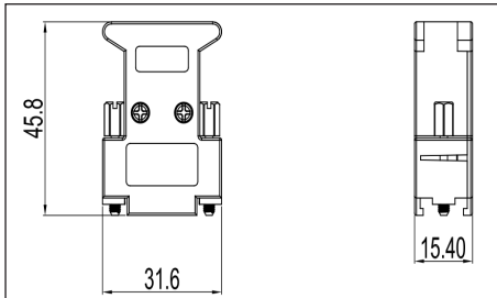
9-WAY
