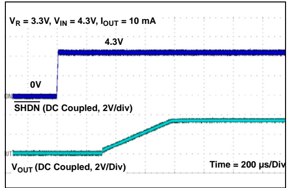
FIGURE 2-46: Start-up from SHDN (MCP1811X, V_R = 3.3\text{V} ).
