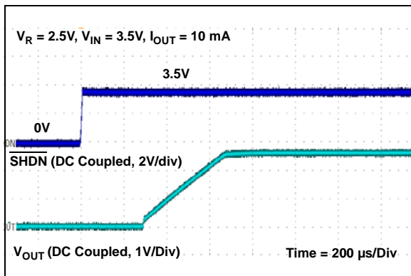
FIGURE 2-45: Start-up from SHDN (MCP1812X, V_R = 2.5\text{V} ).
