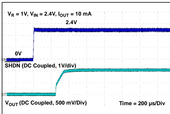
FIGURE 2-44: Start-up from SHDN (MCP1812X, V_R = 1.0\text{V} ).
