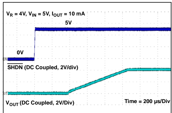
FIGURE 2-47: Start-up from SHDN (MCP1811X, V_R = 4.0\text{V} ).
