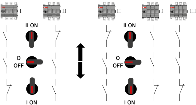
Change-over switches
