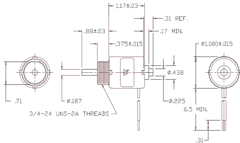
Solenoid shown energized with plunger fully seated in extended position Supplied with mounting bracket, hex nut and lock washer shipped loose
