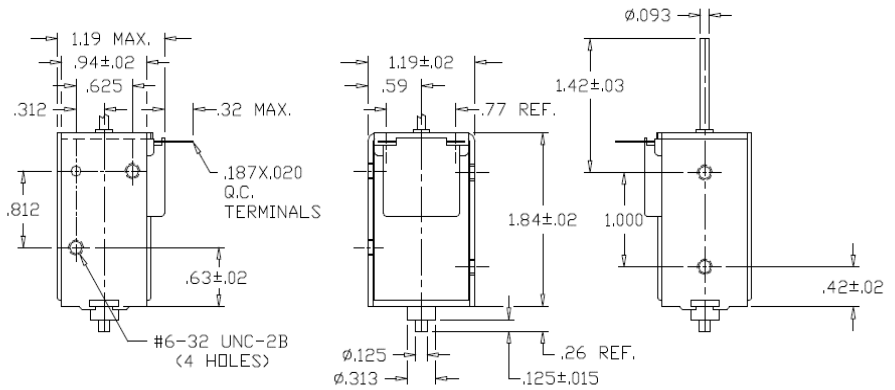
Solenoid shown energized with plunger fully seated in extended position
