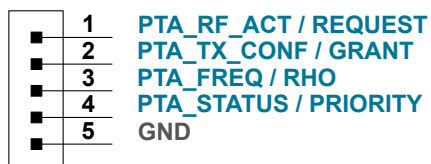
Figure 4.5. PTA Connector
