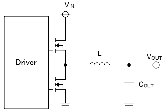
Figure 63. Output LC Filter Circuit
