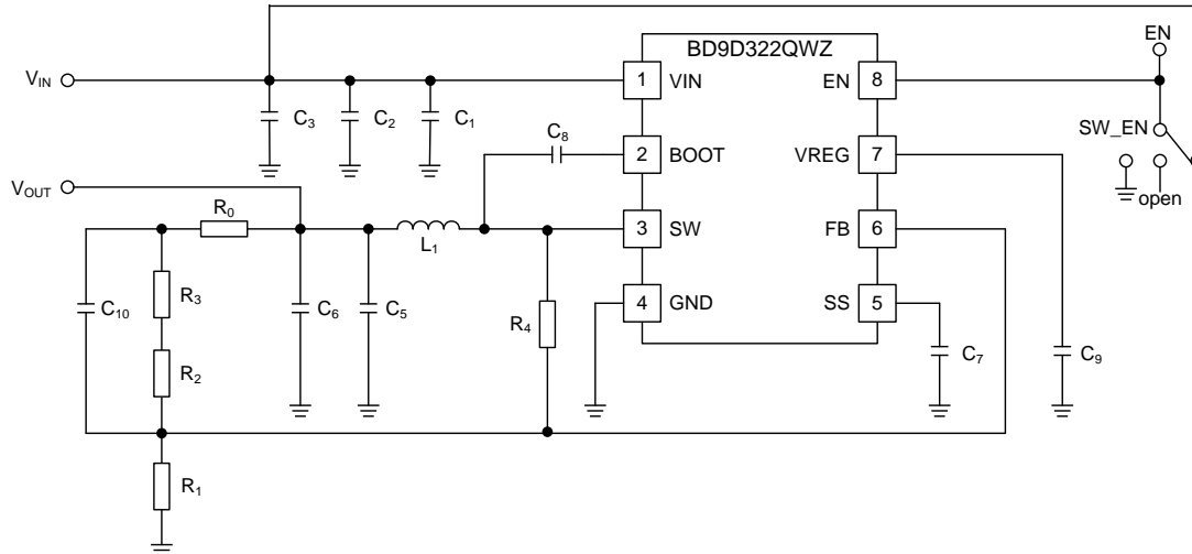
Figure 47. Application Circuit
