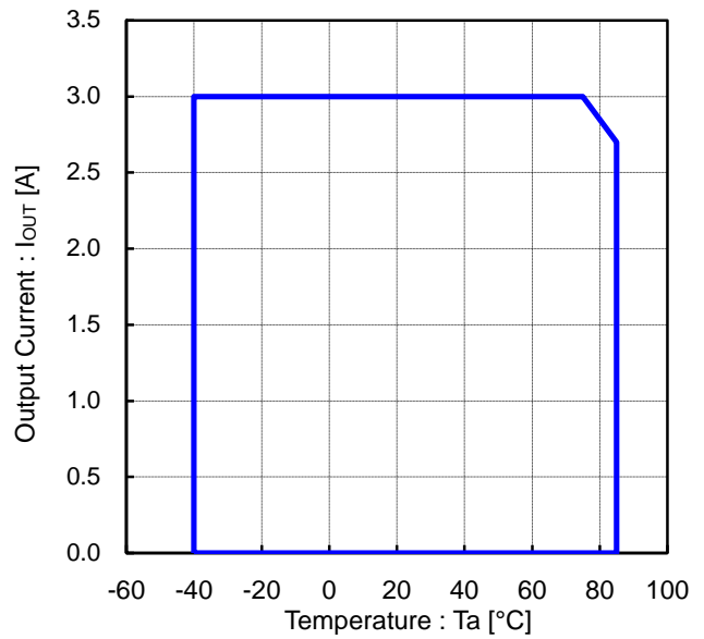
Figure 22. Operational Range V_{IN} = 12V , V_{OUT} = 5V ( T_j < 150^\circ C ) (Measured on FR-4 board 67.5 mm x 67.5 mm, Copper Thickness : Top and Bottom 70 \mu m , 2 Internal Layers 35 \mu m )
