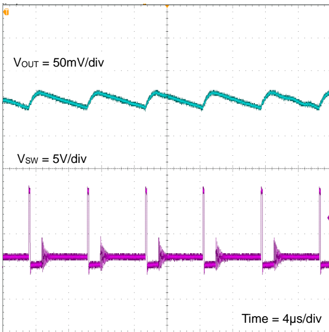
Figure 60. V_{OUT} Ripple I_{OUT} = 0.1A ( V_{IN}=12V , V_{OUT}=1.2V )
