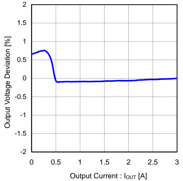
Figure 34. V OUT Load Regulation (V IN =12V, V OUT =1.8V)
