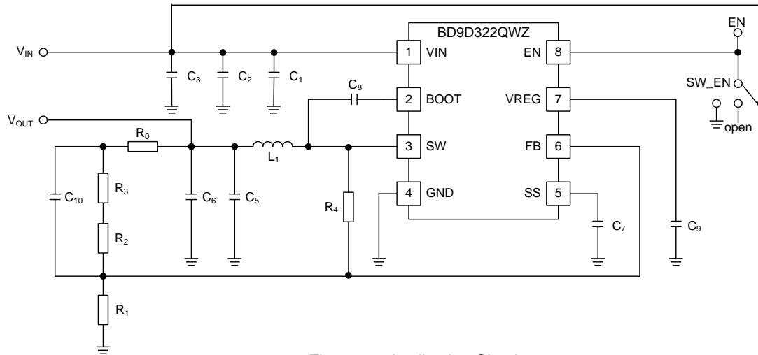
Figure 57. Application Circuit
