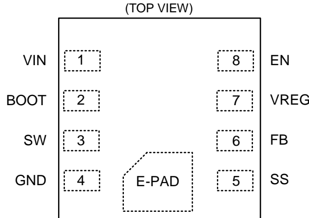
Figure 2. Pin Configuration
