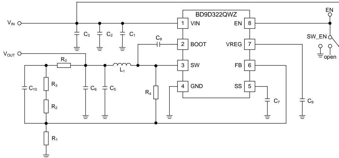
Figure 52. Application Circuit
