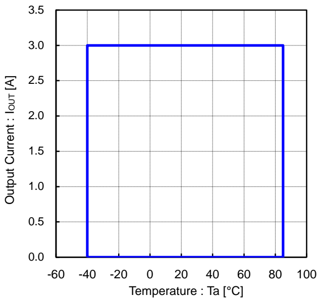
Figure 21. Operational Range V_{IN} = 12V , V_{OUT} = 1V ( T_j < 150^\circ C ) (Measured on FR-4 board 67.5 mm x 67.5 mm, Copper Thickness : Top and Bottom 70 \mu m , 2 Internal Layers 35 \mu m )
