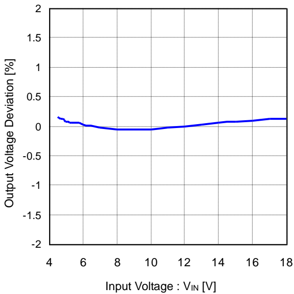
Figure 33. V OUT Line Regulation (V OUT =1.8V, I OUT =1A)
