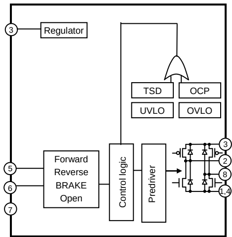
Figure 4. Block Diagram
